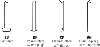
Figure 3-5 Sanitary Sensor Pipe
