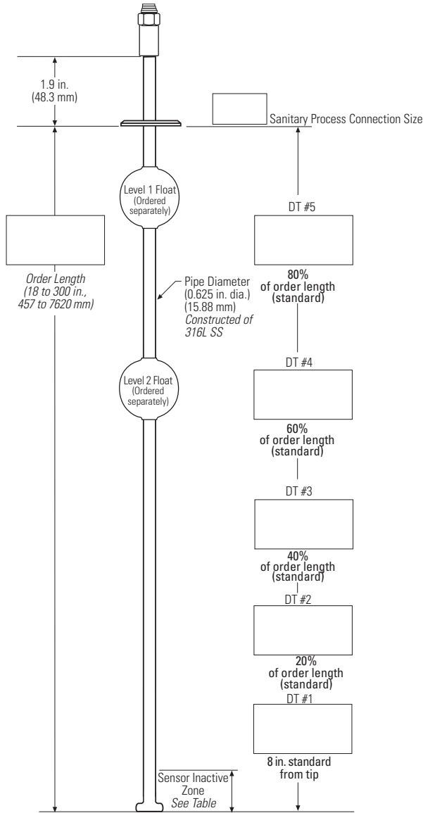
Figure 3-5 Sanitary Sensor Pipe
